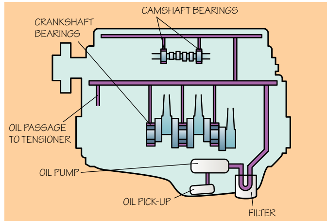
Lubrication system components
