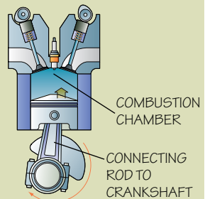
Compression stroke
