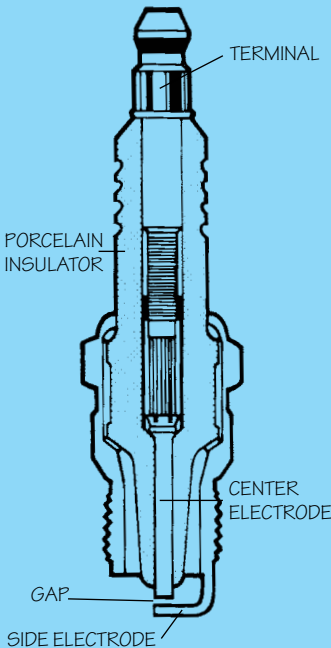
Spark plug construction
