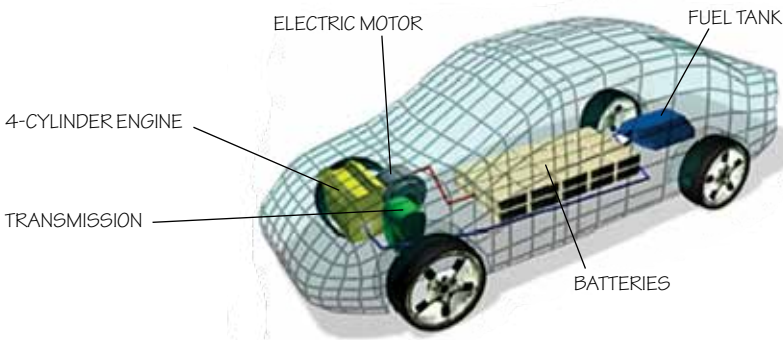
Gasoline-electric parallel hybrid drive train
