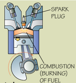
Power stroke
