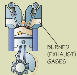
Exhaust stroke
