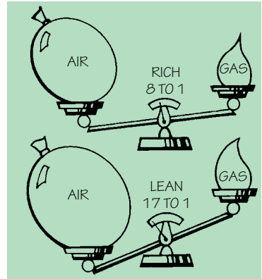
Different air-fuel ratios are required for different operating conditions.
